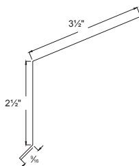
18 Denver Eave
