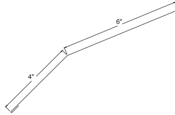
5 Gambrel Trim
