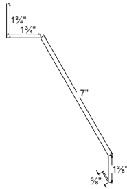
8 Track Cover
