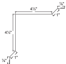
11 Inside Corner
