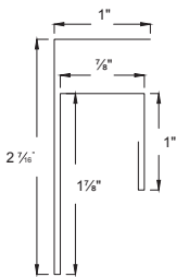
16 F&J Channel
