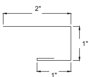
16 J Channel
