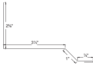
4 Universal Sidewall
